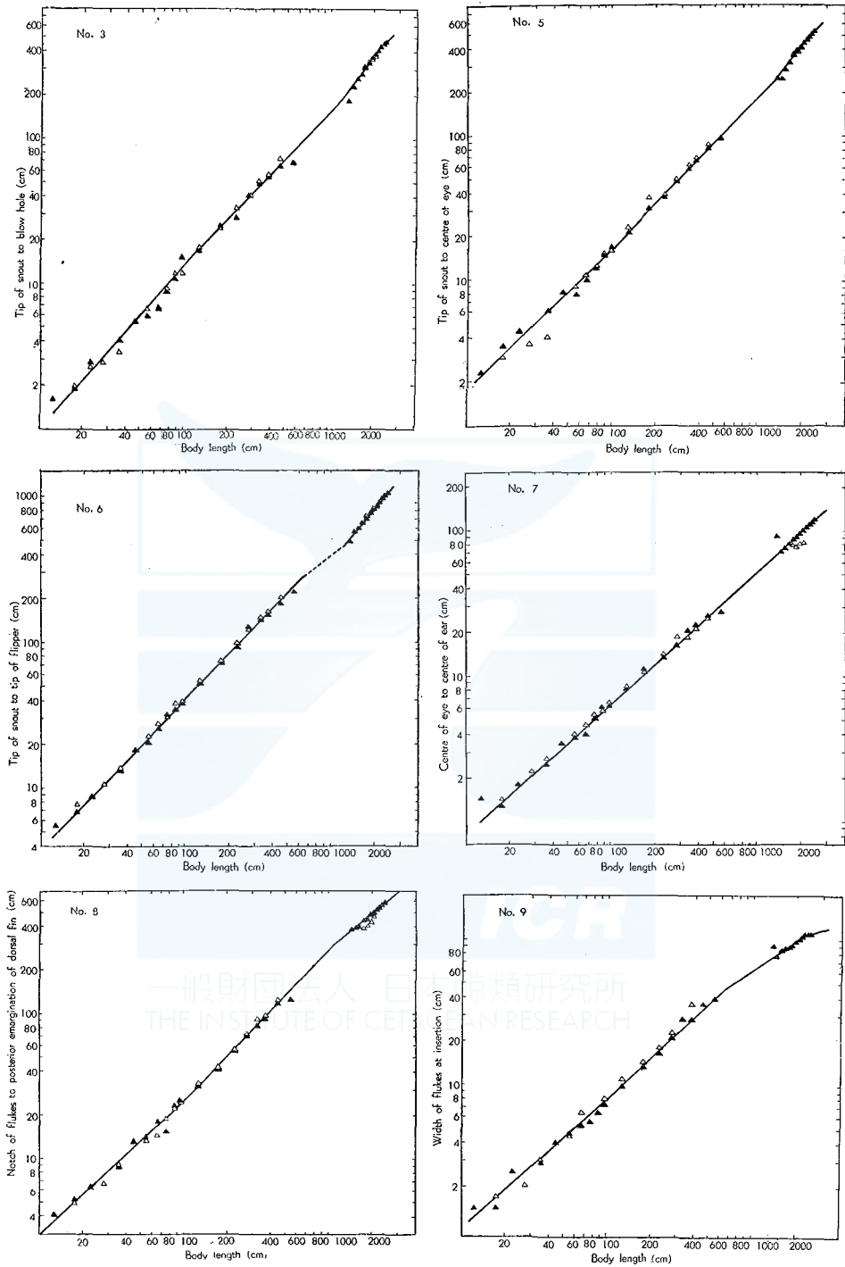
Fig. 3. Comparison of the relative growths between the Antarctic and the North Pacific fin whales.
