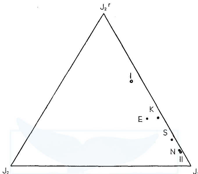
Fig. 9. Relative positions of the local populations of the North Pacific Finback whales in the triangular coordinates, expressed through the three allele B system of J_u blood group.
