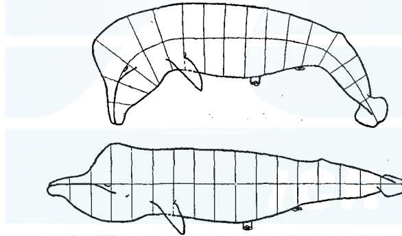
Fig. 1. Modification of the shape of small foetus for the measurement of body proportions. Female fin whale foetus, 18.6 cm long.
