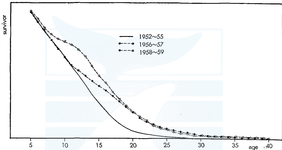
Fig.5. Age composition of the North Pacific Fin whales, estimated from distribution of frequency of corpus albicans of pregnant females.
