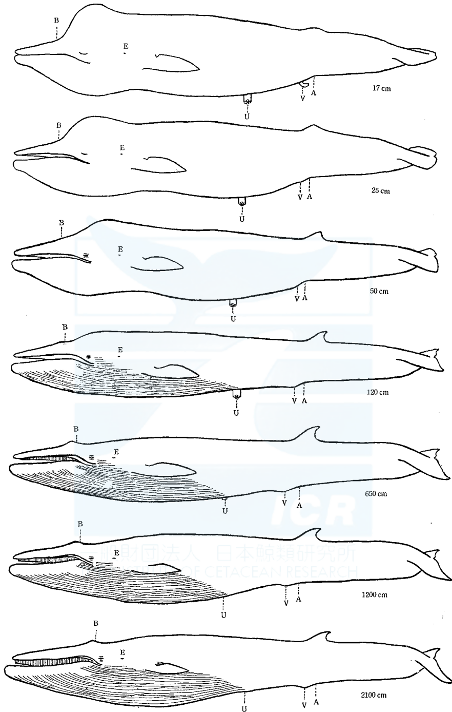
Fig. 13. Variation of the external form in the female fin whales. A: Anus, B: Blow hole, E: Ear, U: Umbilicus, V: Vagina opening
