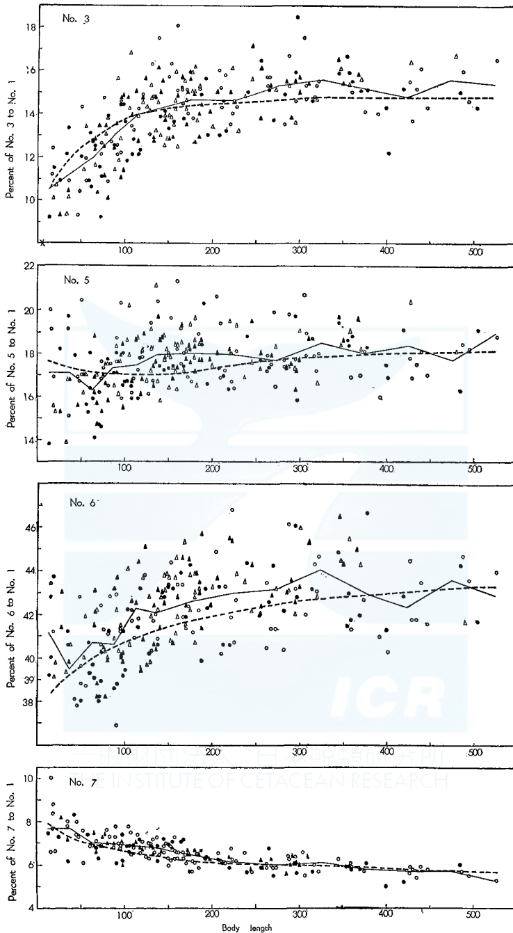
Fig. 9. Variation of the proportions of measurements in the fin whale fetuses. Open circle: Antarctic female, closed circle: Antarctic male, Open triangle: North Pacific female, closed circle: North Pacific male, Solid line: Mean proportion in each body length class, Broken line: Proportion calculated from allometry.
