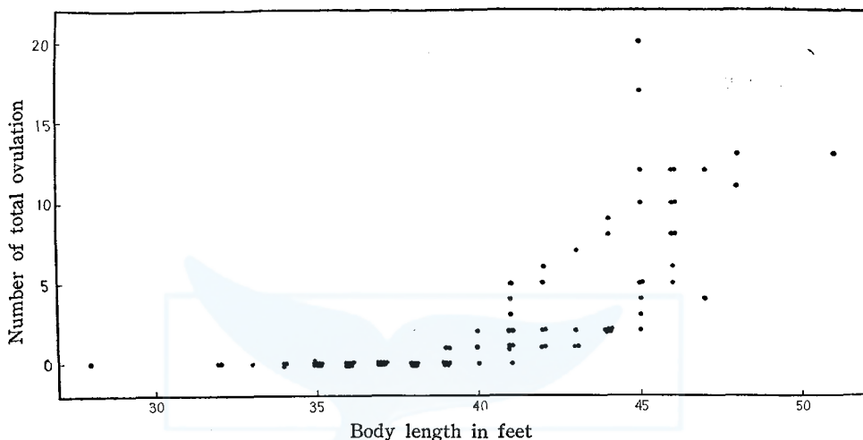
Fig. 5. Relation between body length and total ovulation number.
