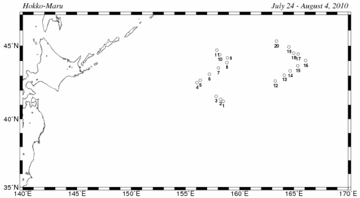
Fig. 1. Station map observed by R/V Hokko-Mar in 24 th July to 4 th August 2010.
