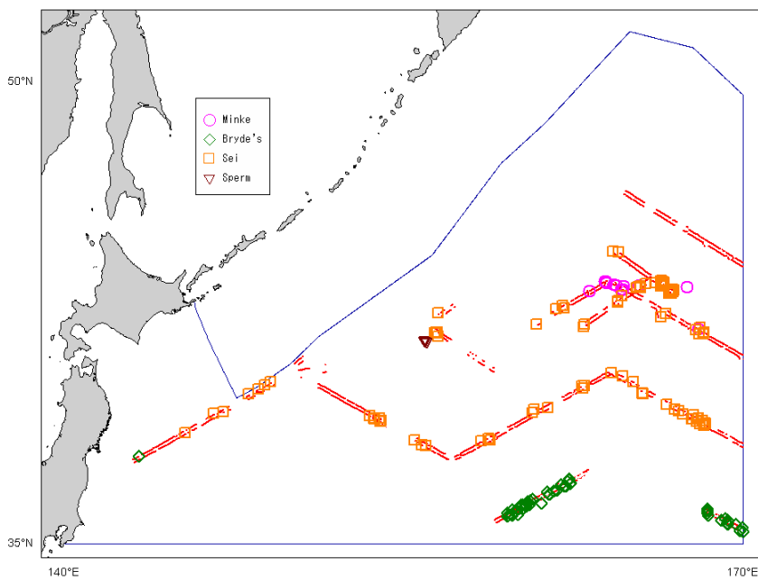
Fig. 4. The Sighting positions of the sampled common minke whale (pink circle), sei (orange square), Bryde's (green diamond) and sperm (brown triangle) whales. Two blocks show the cooperative survey areas of prey species and whale sampling survey.
