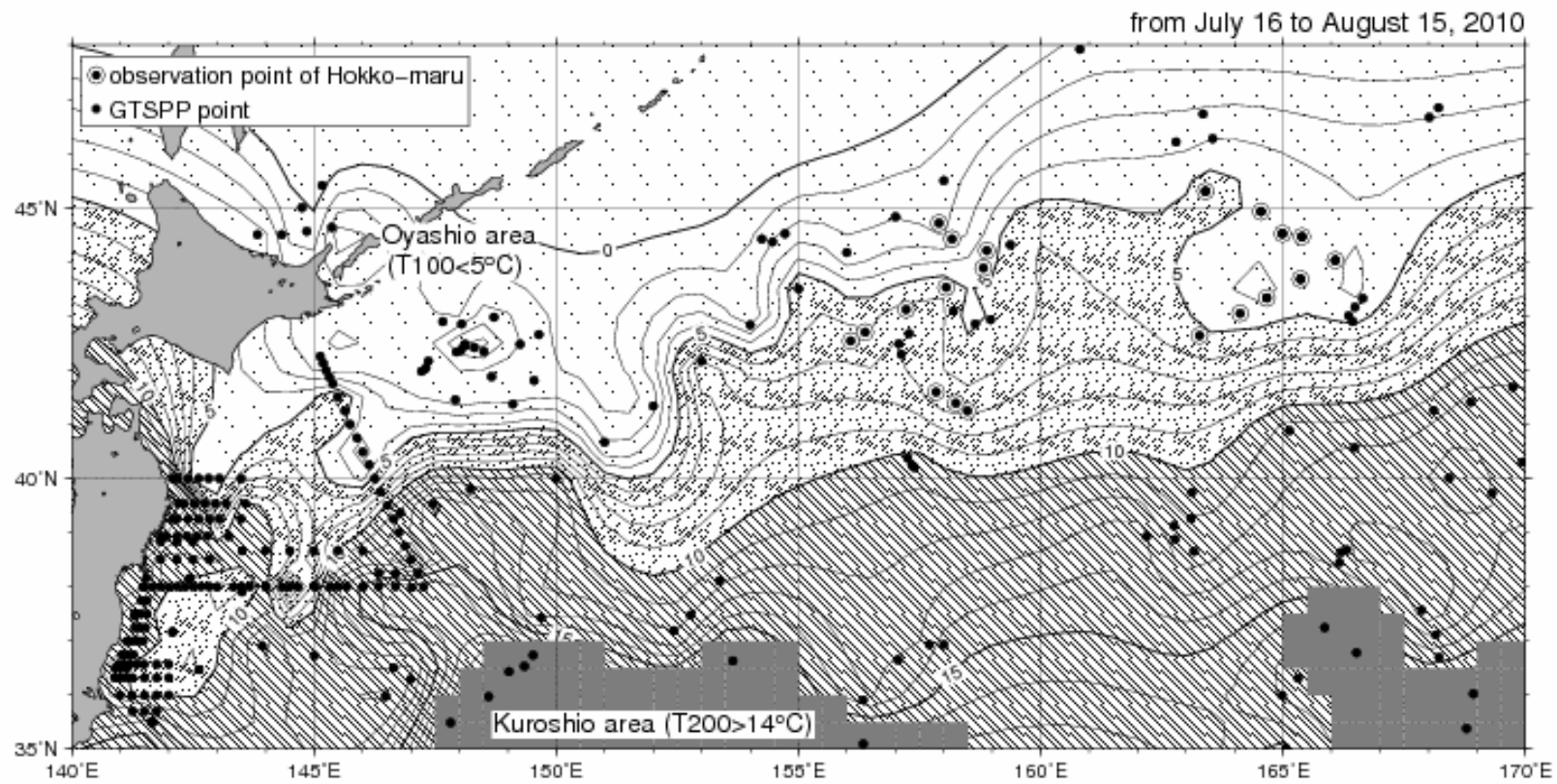
Fig. 3. Schematic hydrographic map in the western North Pacific between July 16 and August 15 in 2010 with station map observed by R/V Hokko-Maru and reported to GTSP.
