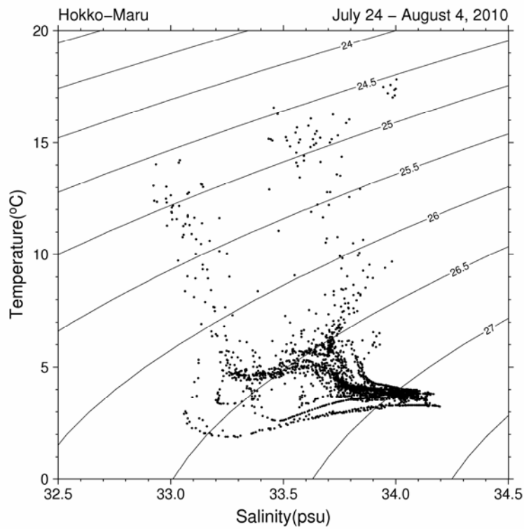
Fig. 2. Temperature-Salinity diagrams using CTD station data observed by R/V Hokko-Mar . Each thin line in this figure denotes a density line of sigma-t.
